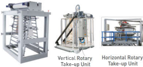
⑤ Take-up Unit
